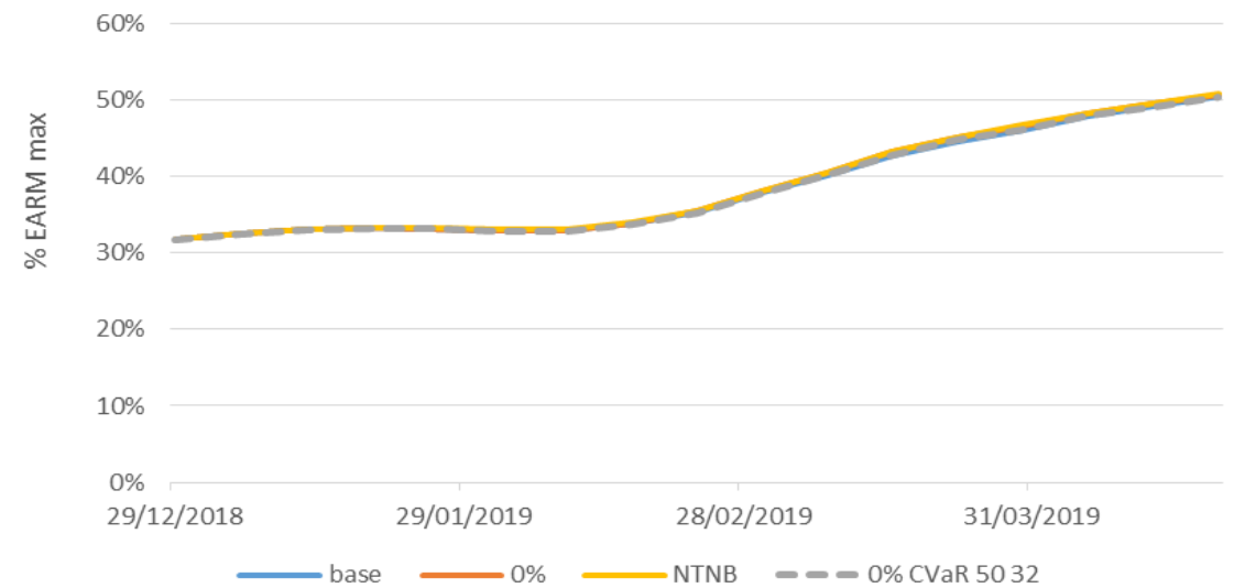
EARM SIN
